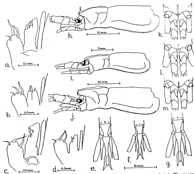
Fig. 9. The bathypelagic giant euphausiids. Male copulatory organs of (a) Thysanopoda spiniicaudata , 104 mm. in length; (b) Thysanopoda egregia , 43 mm. in length; (c) Thysanopoda cornuta , 95 mm. in length; (d) T. cornuta , 50 mm. in length. Telson and uropods, in dorsal view, of the largest male specimens of (e) T. spiniicaudata , (f) T. egregia , (g) T. cornuta . Lateral view of antennal peduncles and carapace of the same large specimens of (h) T. spiniicaudata , (i) T. egregia , (j) T. cornuta . Dorsal view of frontal plate and antennal peduncles of the same specimens of (k) T. spiniicaudata , (l) T. egregia , (m) T. cornuta .
